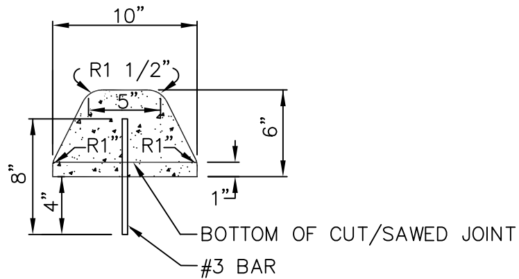
SECTION
