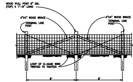
PULL POST BRACE PANEL DETAIL NO SCALE
