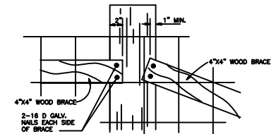
DAP DETAIL NO SCALE
