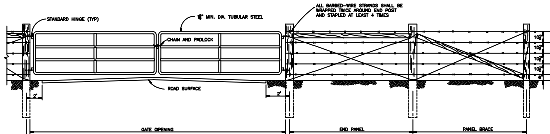
TYPICAL PANEL GATE DETAIL NO SCALE
