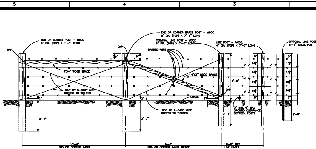
① TYPICAL LAYOUT - 5 STRAND BARBED WIRE FENCE NO SCALE
