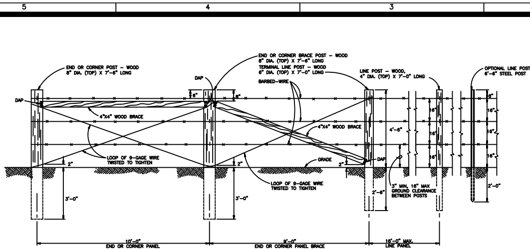
① TYPICAL LAYOUT - 3 STRAND BARBED WIRE FENCE NO SCALE
