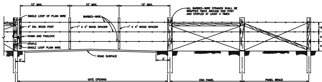
TYPICAL BARBED-WIRE DROP GATE DETAIL NO SCALE
