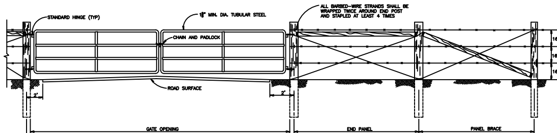
TYPICAL PANEL GATE DETAIL NO SCALE
