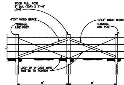
PULL POST BRACE PANEL DETAIL NO SCALE
