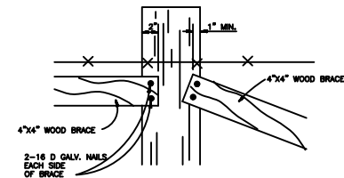
DAP DETAIL NO SCALE
