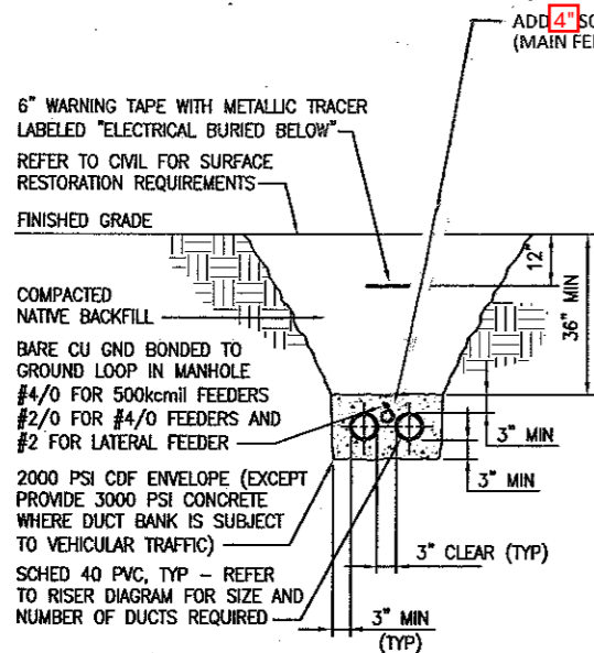
1 TYPICAL DETAIL MEDIUM-VOLTAGE POWER TRENCH SCALE: NONE
