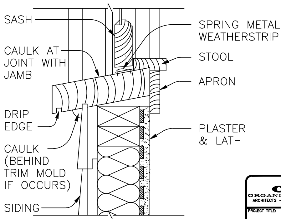
SECTION THROUGH TYPICAL SILL
