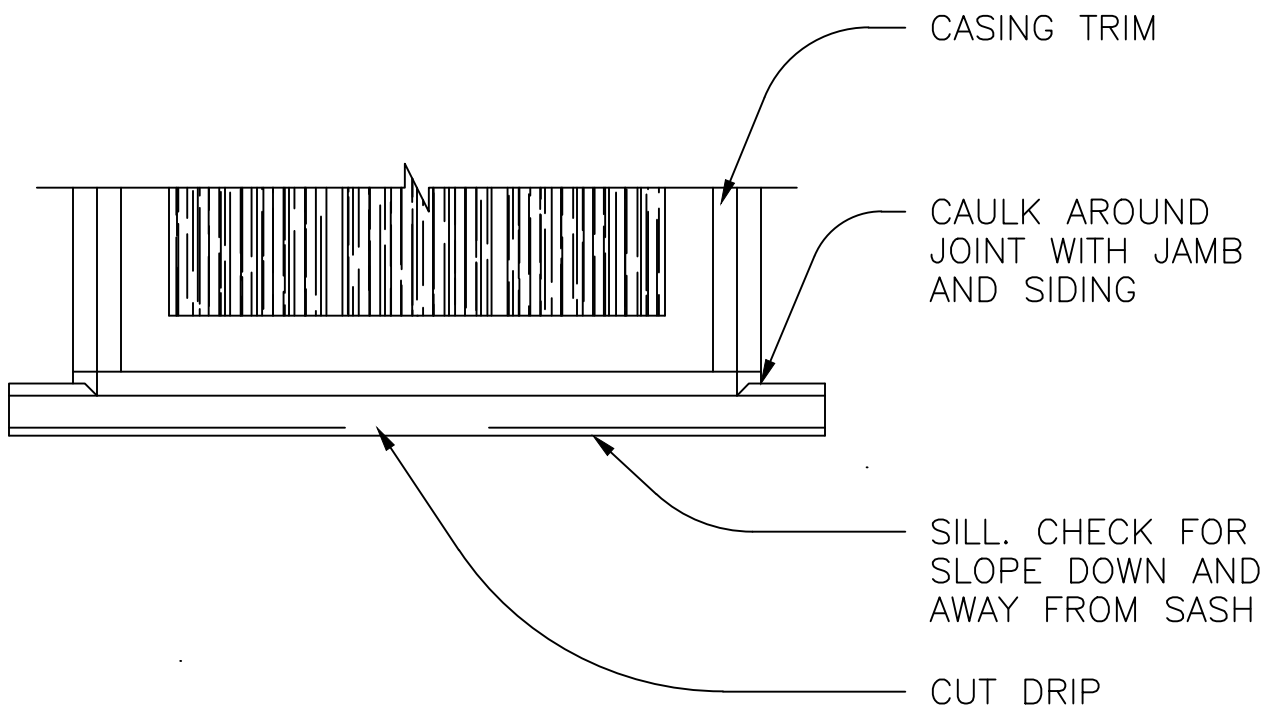
ELEVATION – TYPICAL EXTERIOR WINDOW SILL
