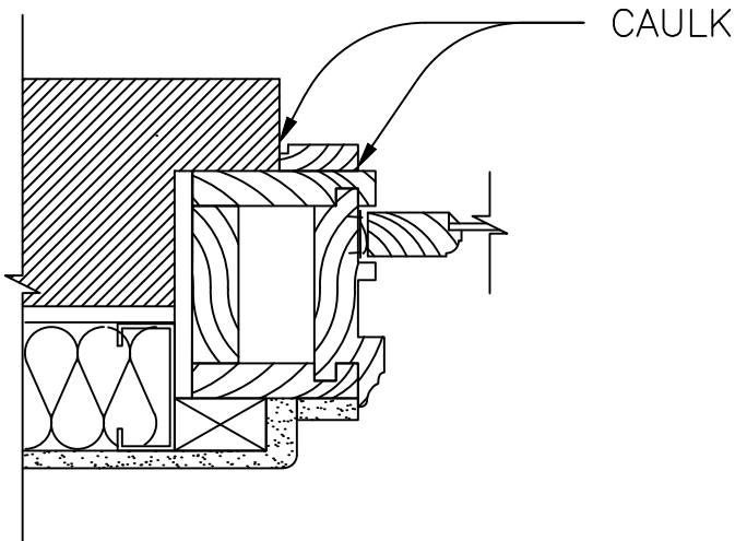
SPRING "V" BRONZE TYPE JAMB
