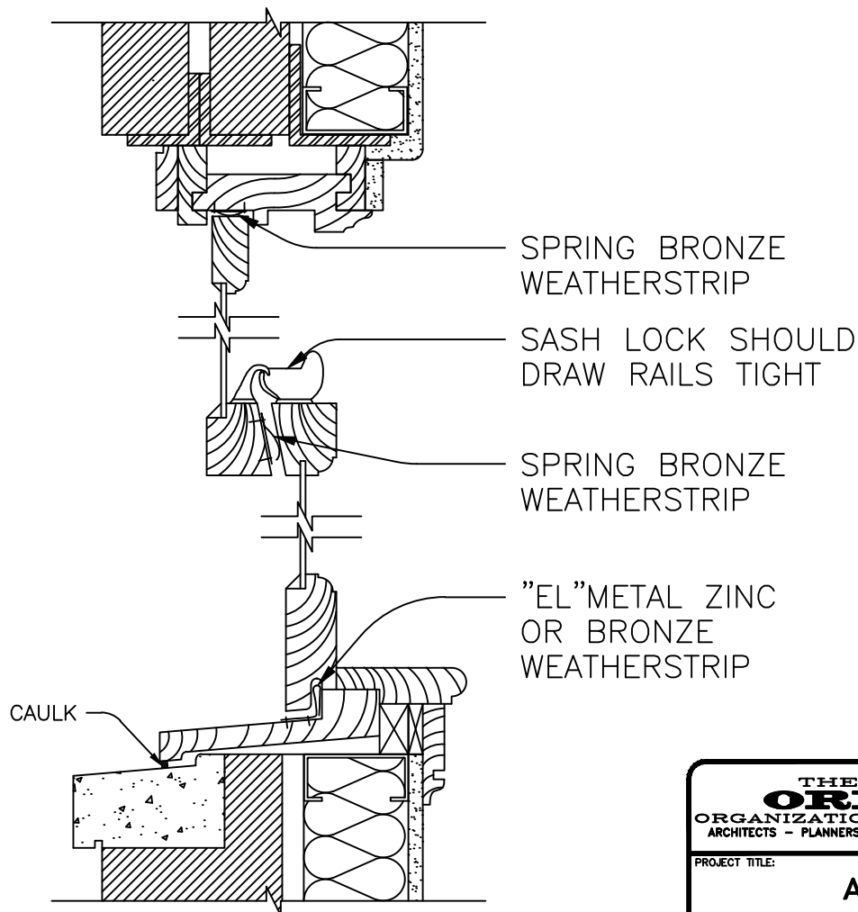
HEAD/MEETING RAIL/SILL
