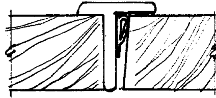
COMPRESSION BULB APPLIED TO ASTRAGAL
