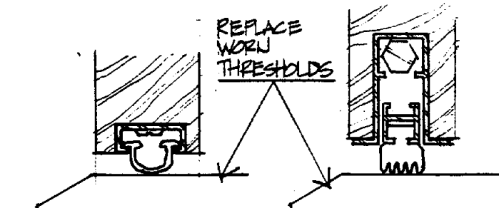
RECESSED NEOPRENE OR VINYL
