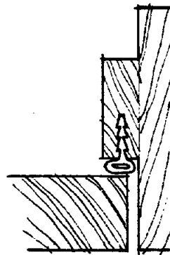
SET IN GROOVE IN STOP
