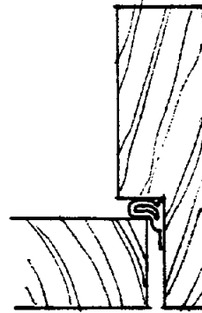
SELF-ADHESIVE SILICON COMPRESSION BULB. CAN ALSO BE APPLIED TO ASTRAGAL
