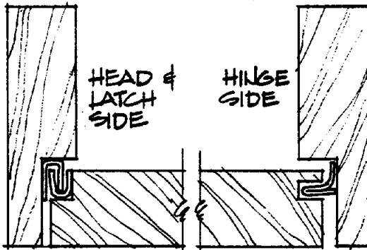
INTERLOCKING METAL (REQUIRES MILLING EDGES OF DOOR)
