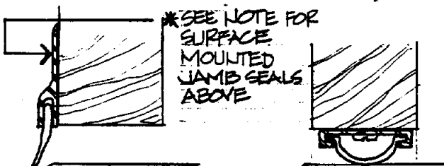
SURFACE MOUNTED PILE OR NEOPRENE SWEEP
