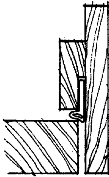
CONCEALED UNDER STOP (RABBIT BACK)
